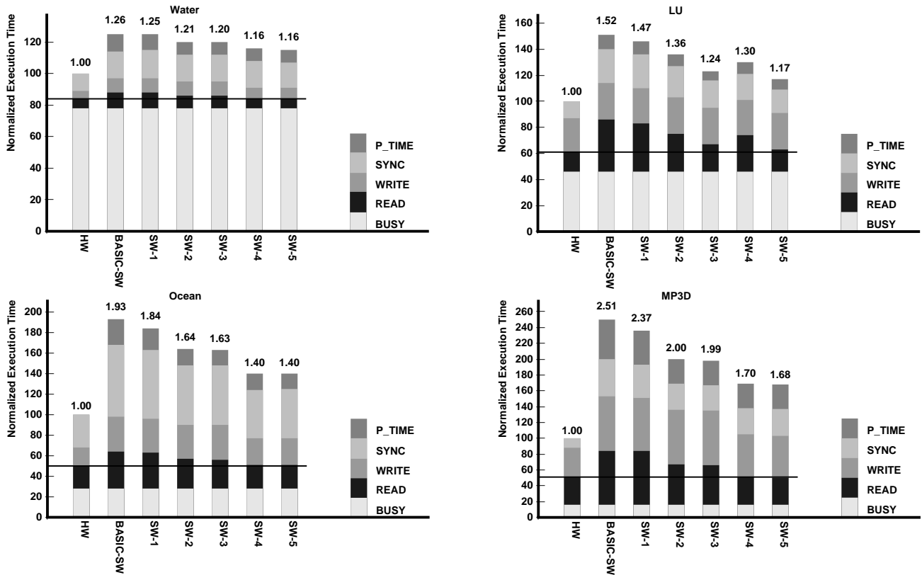
Figure 3: Execution times for the software-only protocols relative to the hardware-only protocol.
