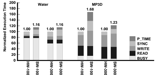
Figure 7: Execution times of SW relative to HW for 100 MHz and 300 MHz processors.
