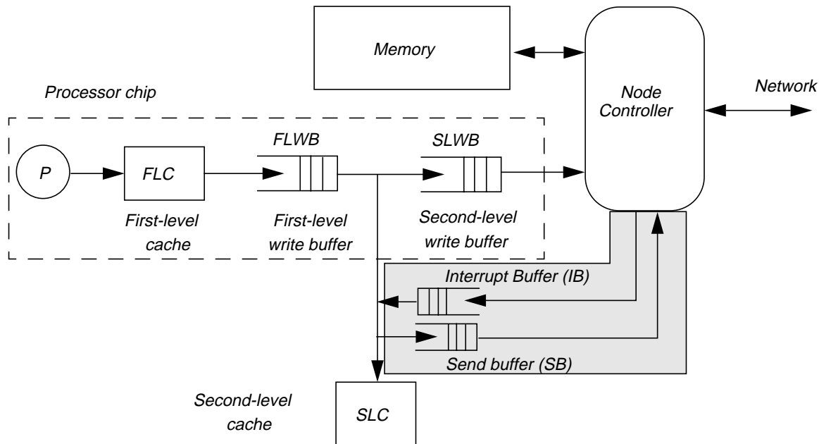
Figure 1: Organization of each processor node. The shaded areas only apply to the software-only protocol that is discussed in Section 2.3.
