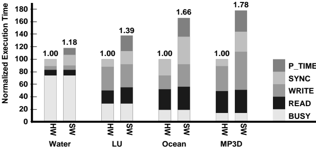
Figure 5: Execution time effects of finite second-level caches (16 Kbyte).
