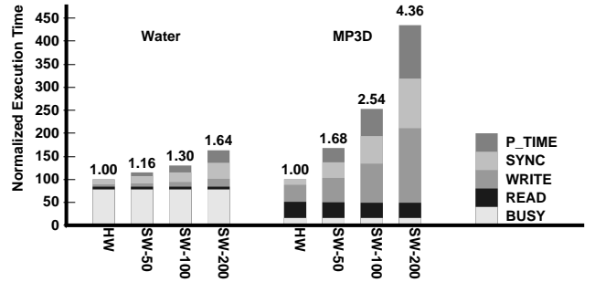
Figure 6: Effects of various protocol execution times.
