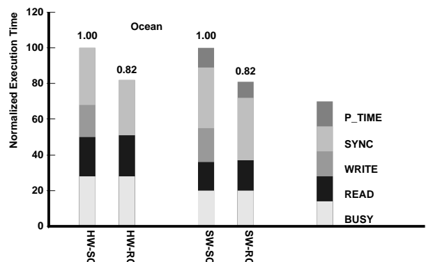
Figure 4: Execution time of HW and SW under sequential consistency (SC) and release consistency (RC) in Ocean. The execution time is normalized for each system to the execution time under sequential consistency.
