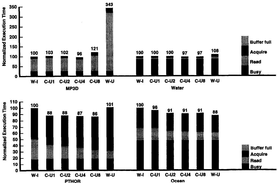
Fig. 9. Normalized execution time under competitive-update with various competitive thresholds.
