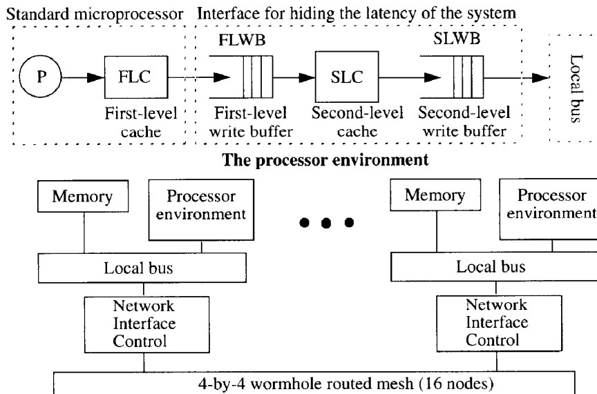
Fig. 3. The processor environment and the simulated architecture.
