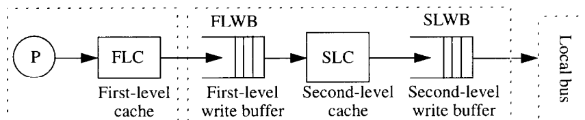
Fig. 2. A two-level cache hierarchy with two separate write buffers and a lockup-free second-level cache.
