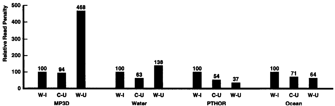
Fig. 6. Relative read penalty under the different coherence policies.
