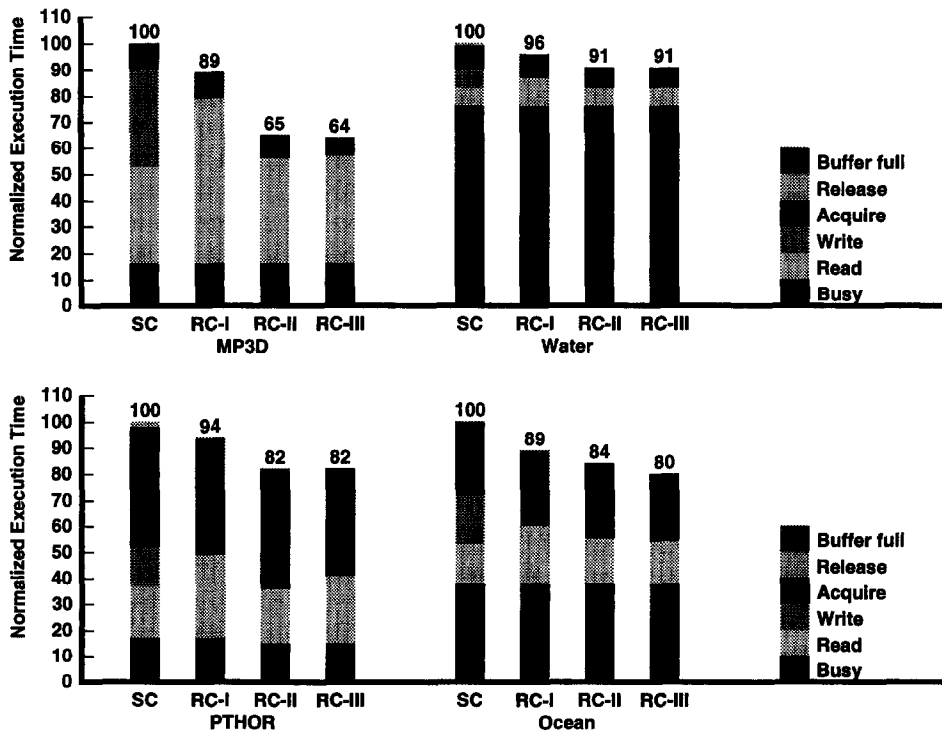
Fig. 7. Normalized execution time of the benchmark applications for the buffering alternatives under write-invalidate.
