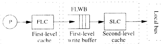
Fig. 1. A basic two-level cache hierarchy.
