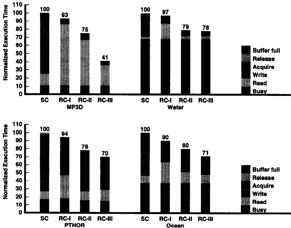
Fig. 8. Normalized execution time of the benchmark applications for the buffering alternatives under competitive-update.
