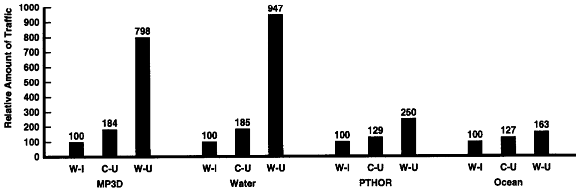
Fig. 5. Relative amount of network traffic generated under the different coherence policies.
