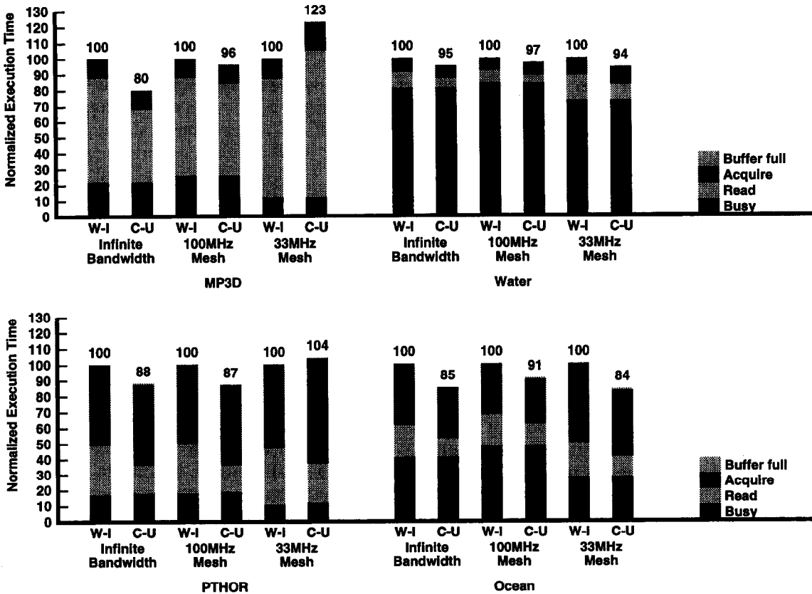
Fig. 10. Effects of varying the capacity and the speed of the network.
